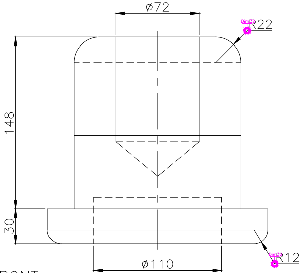
FRONT SCALE 1/3
