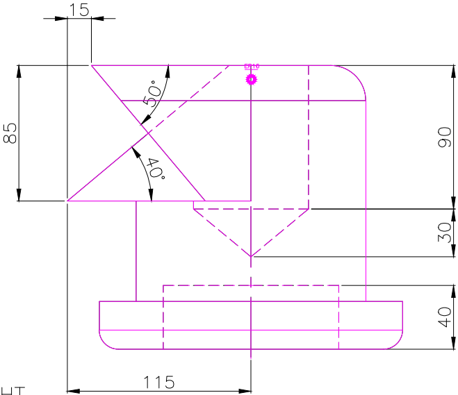
RIGHT SCALE 1/3
