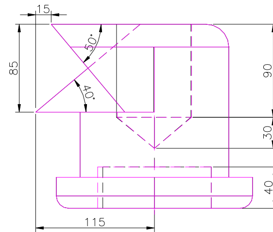
RIGHT SCALE 1/3
