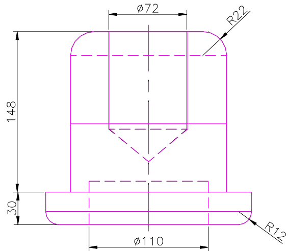
FRONT SCALE 1/3
