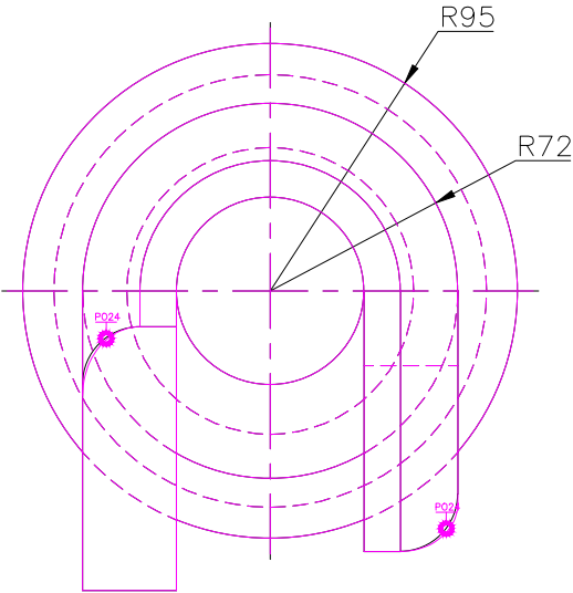
TOP SCALE 1/3
