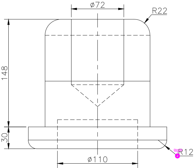
FRONT SCALE 1/3
