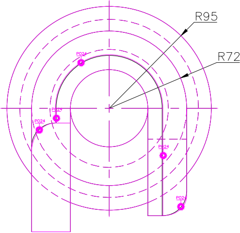
TOP SCALE 1/3
