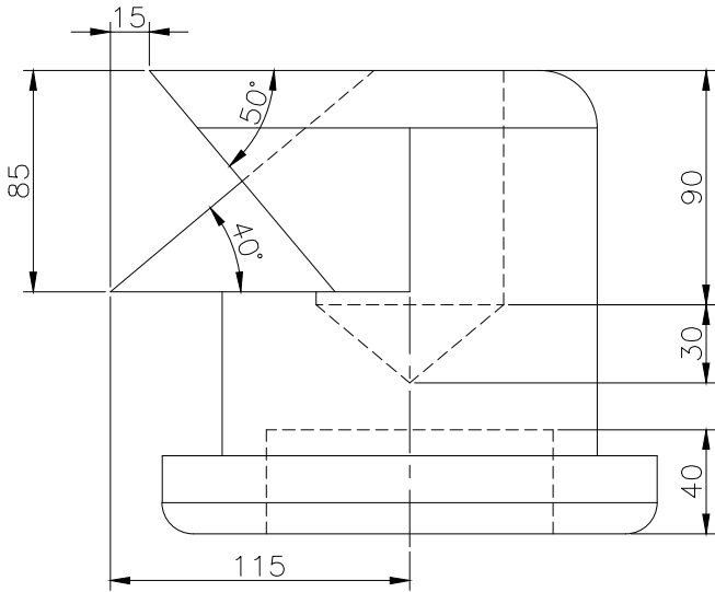
RIGHT SCALE 1/3
