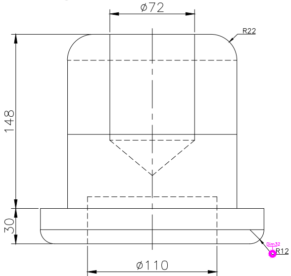
FRONT SCALE 1/3
