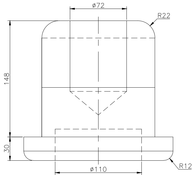
FRONT SCALE 1/3
