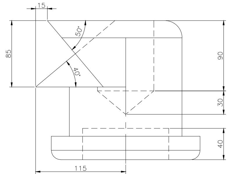
RIGHT SCALE 1/3
