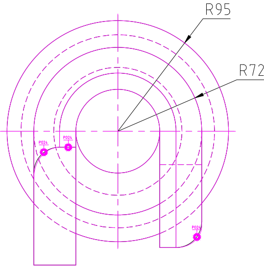
TOP SCALE 1/3
