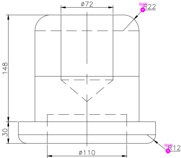
FRONT SCALE 1/3
