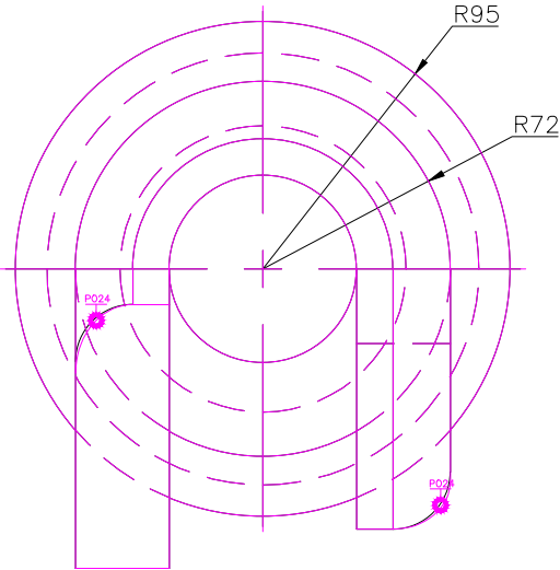
TOP SCALE 1/3
