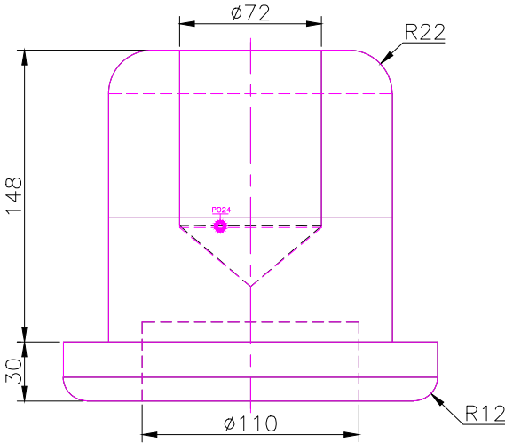
FRONT SCALE 1/3
