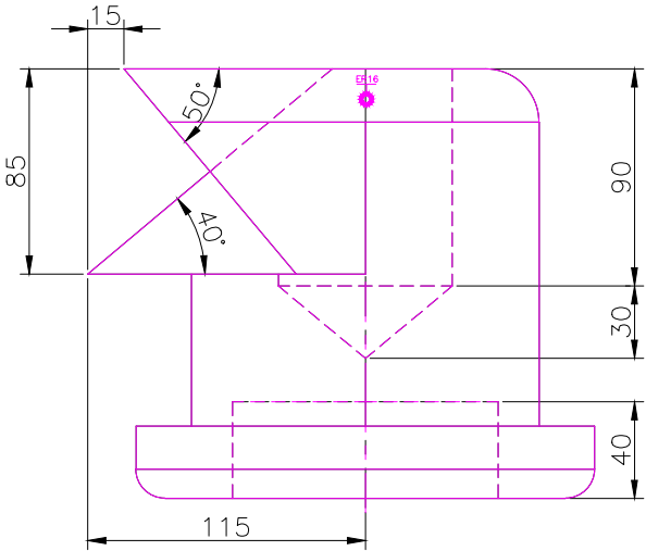
RIGHT SCALE 1/3
