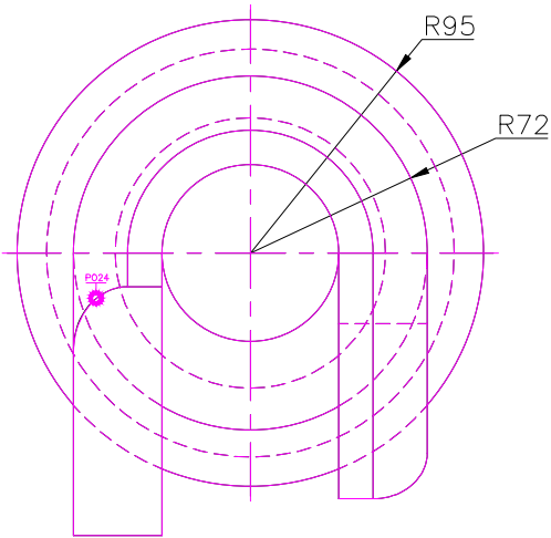
TOP SCALE 1/3
