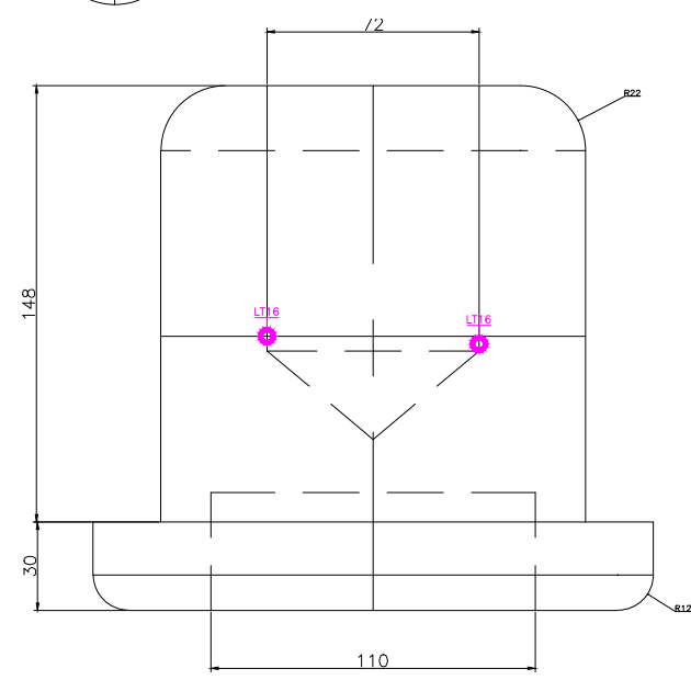
FRONT SCALE 1/3
