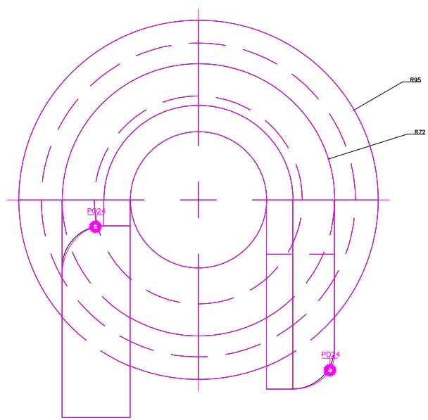
TOP SCALE 1/3
