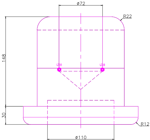
FRONT SCALE 1/3
