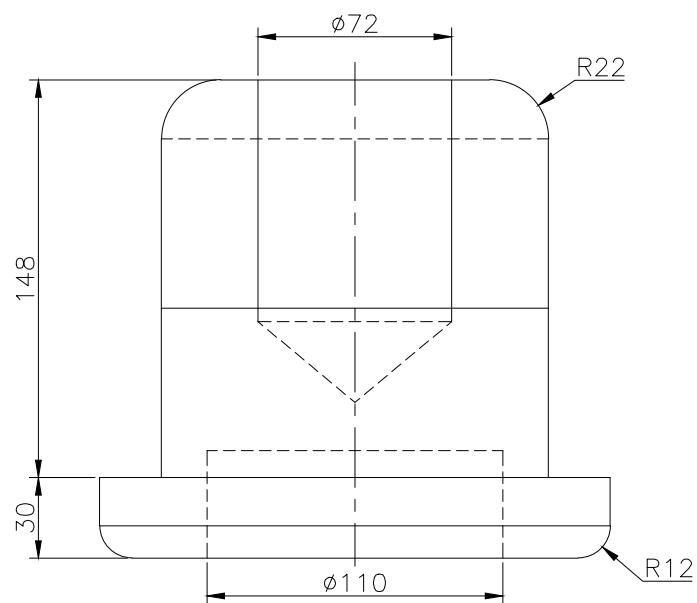
FRONT SCALE 1/3
