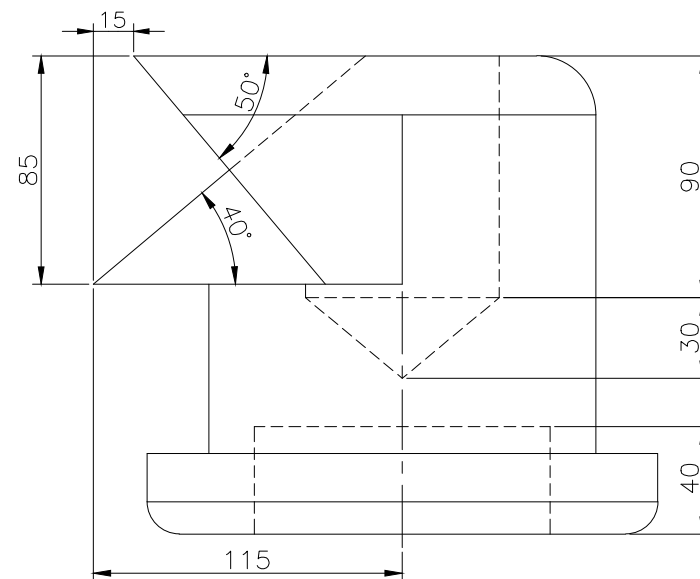
RIGHT SCALE 1/3
