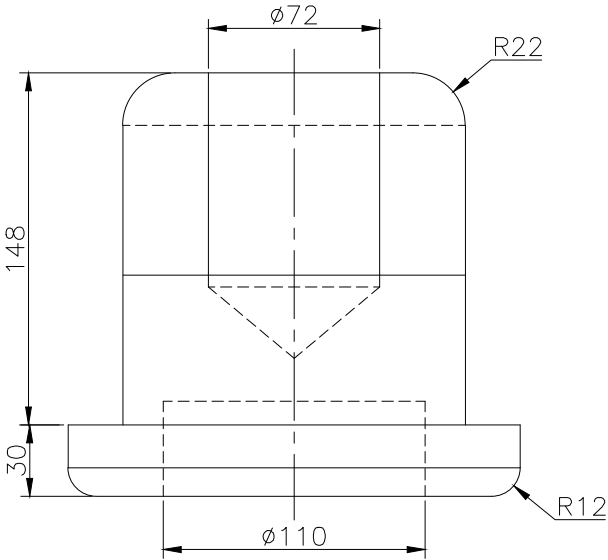
FRONT SCALE 1/3
