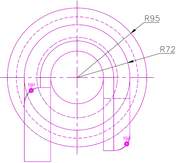
TOP SCALE 1/3
