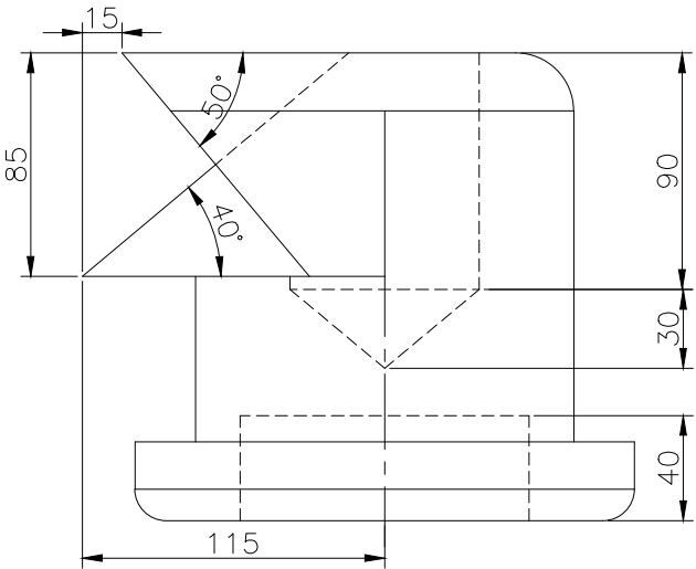
RIGHT SCALE 1/3
