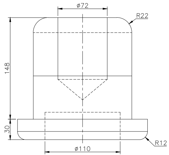
FRONT SCLAE 1/3
