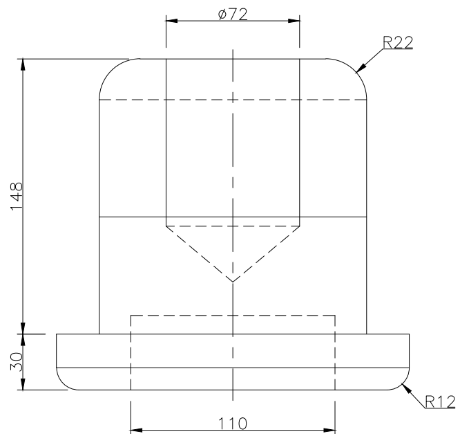
FRONT SCALE : 1/3
