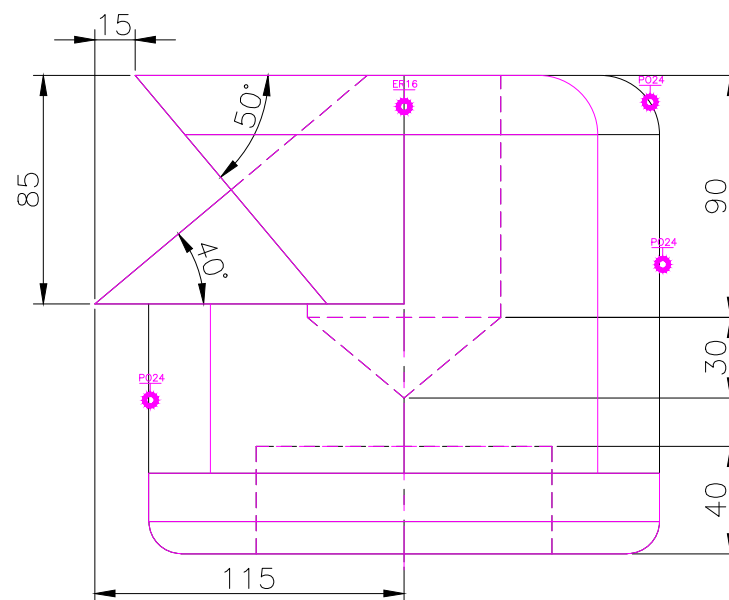
RIGHT SCALE 1/3
