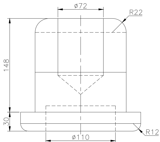
FRONT SCALE 1/3
