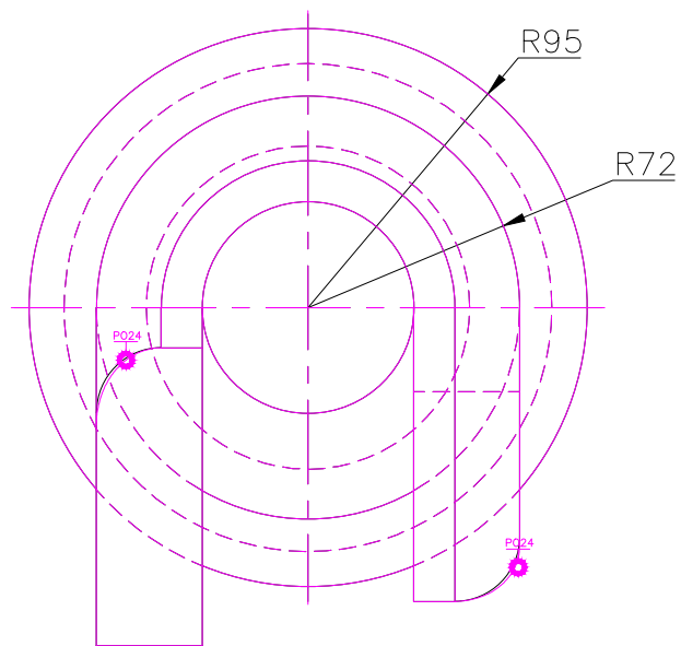
TOP SCALE 1/3
