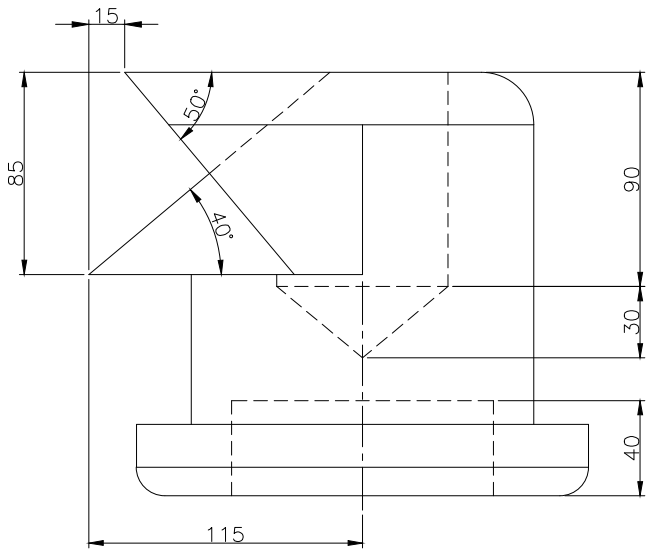
RIGHT SCALE 1/3
