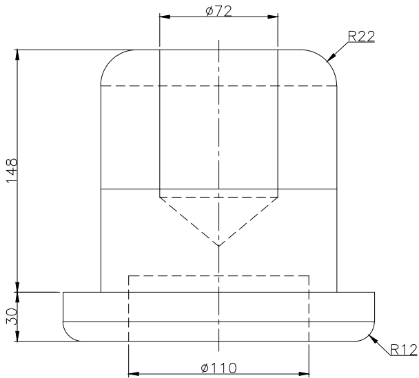
FRONT SCALE 1/3
