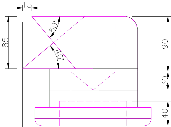
RIGHT SCALE 1/3
