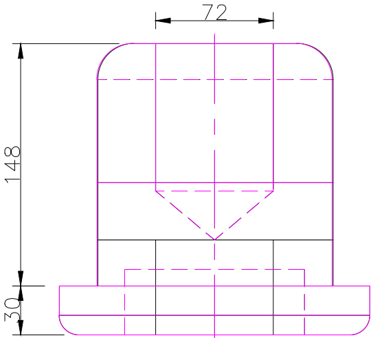
FRONT SCALE 1/3
