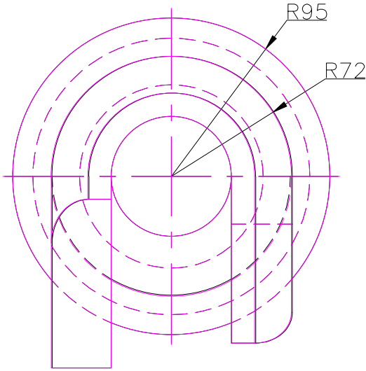
TOP SCALE 1/3
