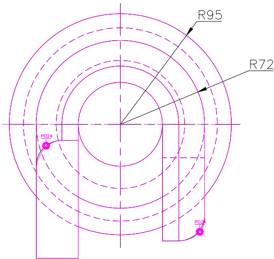
TOP SCALE 1/3
