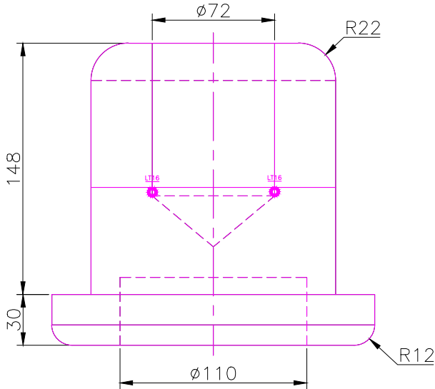
FRONT SCALE 1/3
