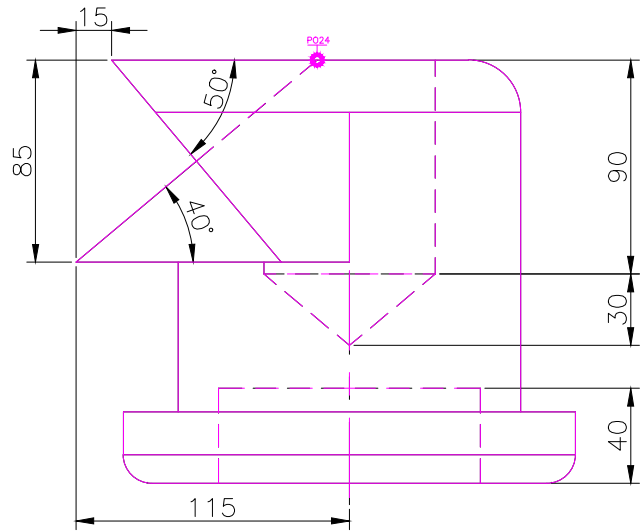
RIGHT SCALE 1/3
