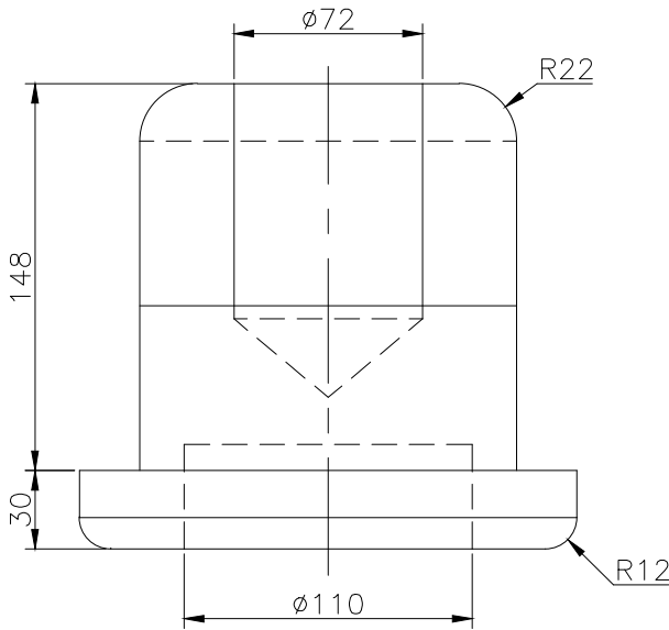
FRONT SCALE 1/3
