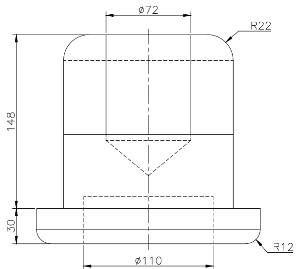
FRONT SCALE 1/3
