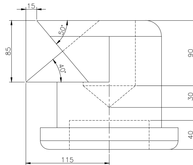
RIGHT SCALE 1/3
