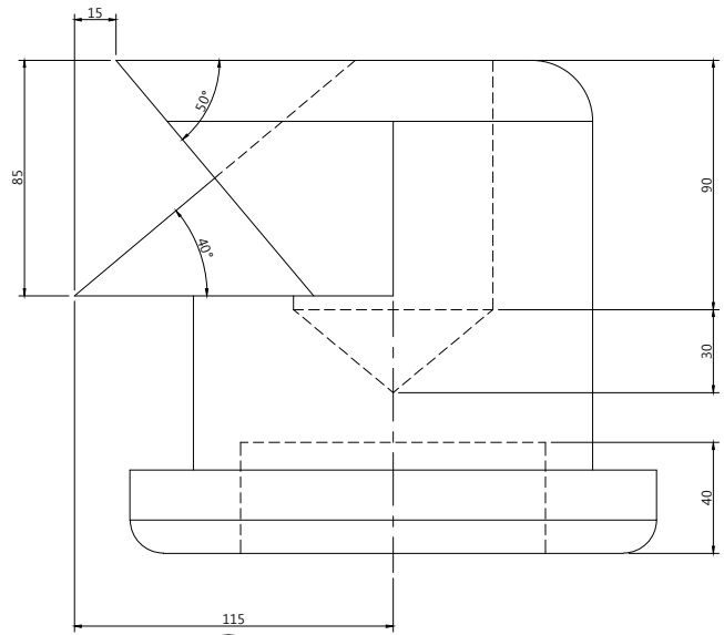
RIGHT SCALE 1/3
