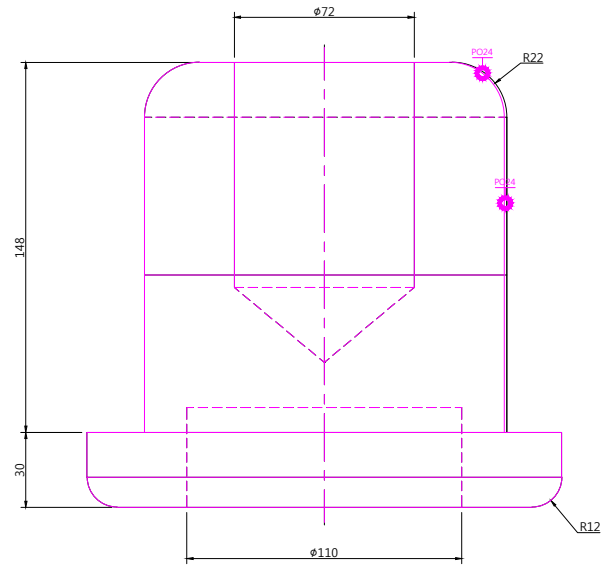
FRONT SCALE 1/3
