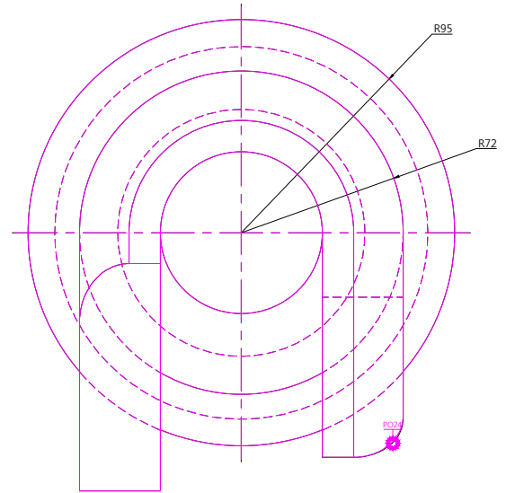
TOP SCALE 1/3
