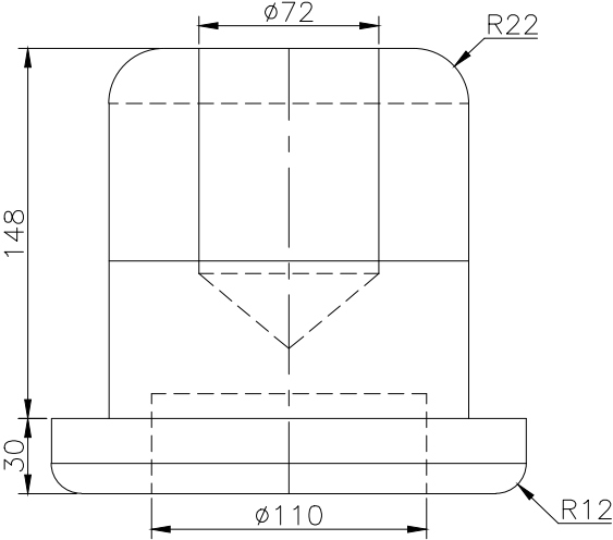
FRONT SCALE 1/3
