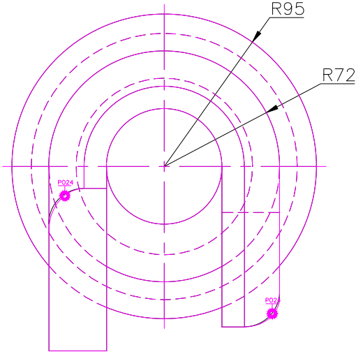
TOP SCALE 1/3
