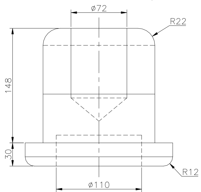
FRONT SCALE 1/3
