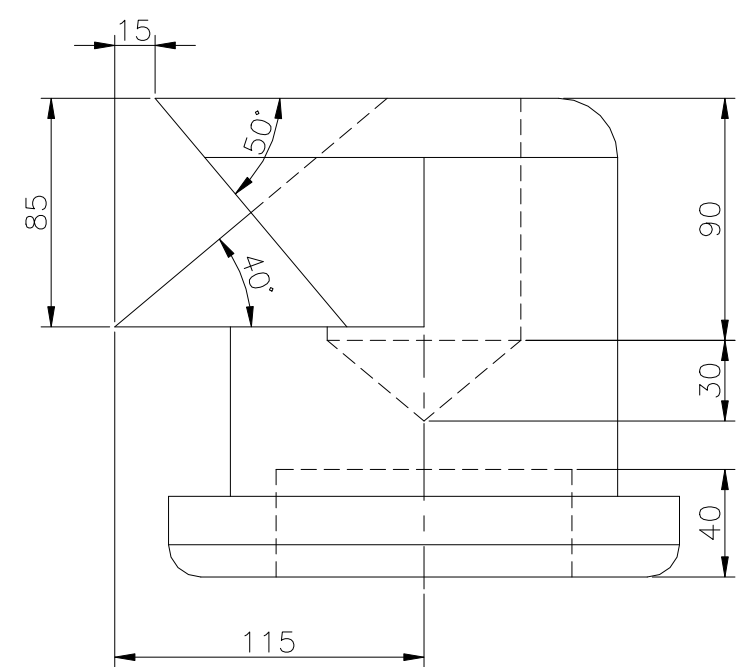
RIGHT SCALE 1/3
