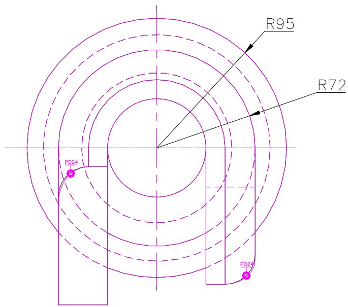
TOP SCALE 1/3
