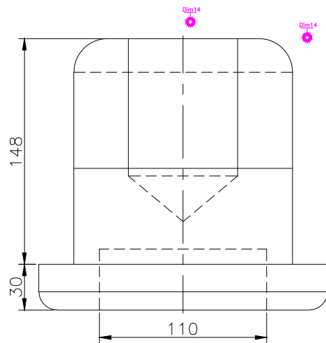
FRONT SCALE 1/3
