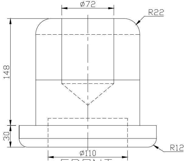
FRONT SCALE 1/3
