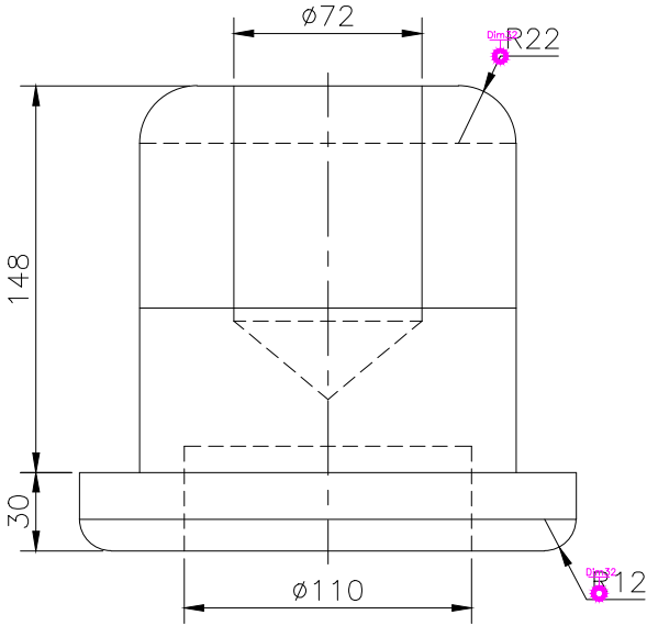
FRONT SCALE 1/3
