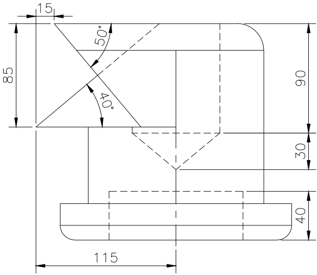
RIGHT SCALE 1/3
