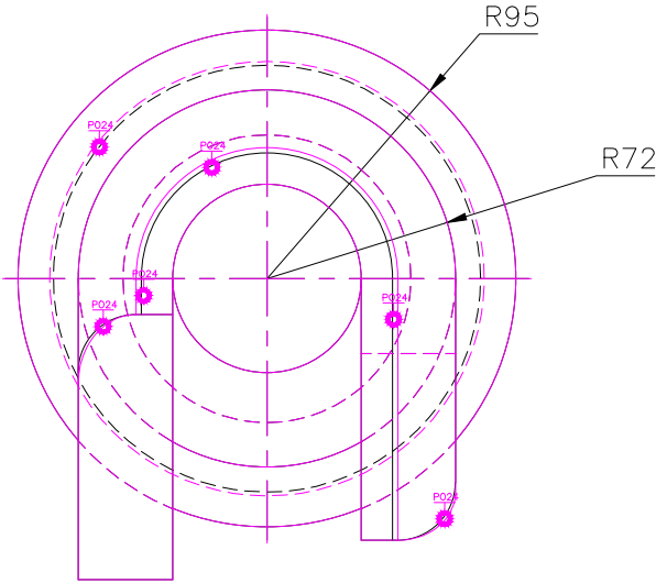
TOP SCALE 1/3
