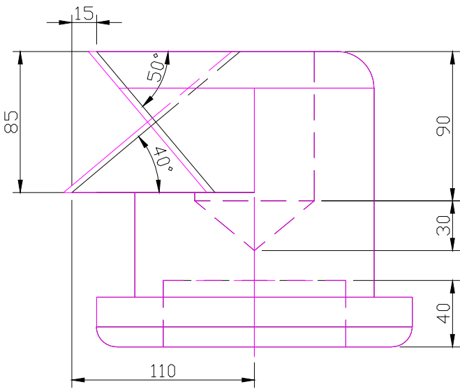
RIGHT SCALE 1/3
