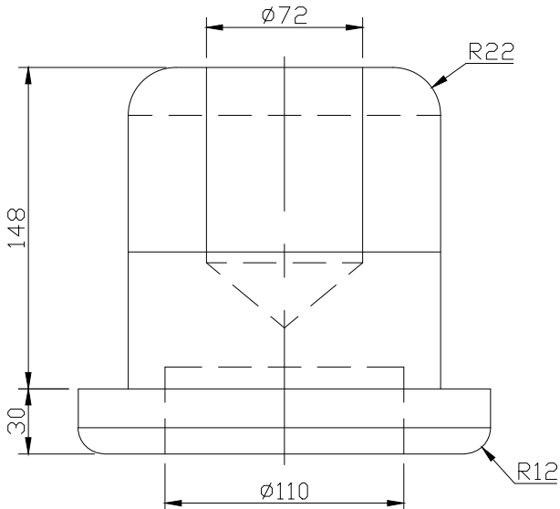
FRONT SCALE 1/3
