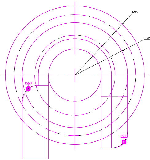
TOP SCALE 1/3
