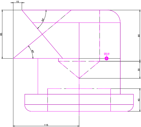
RIGHT SCALE 1/3
