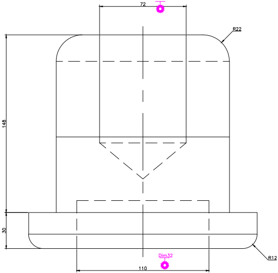
FRONT SCALE 1/3
