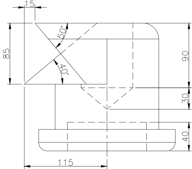
RIGHT SCALE 1/3
