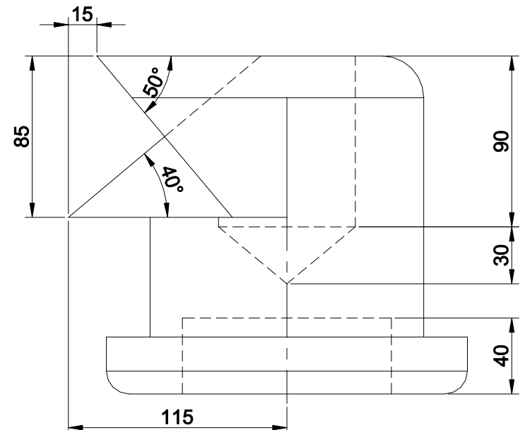
RIGHT SCALE 1/3
