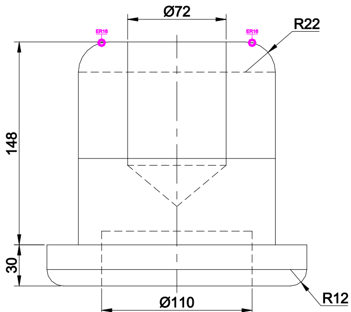
FRONT SCALE 1/3
