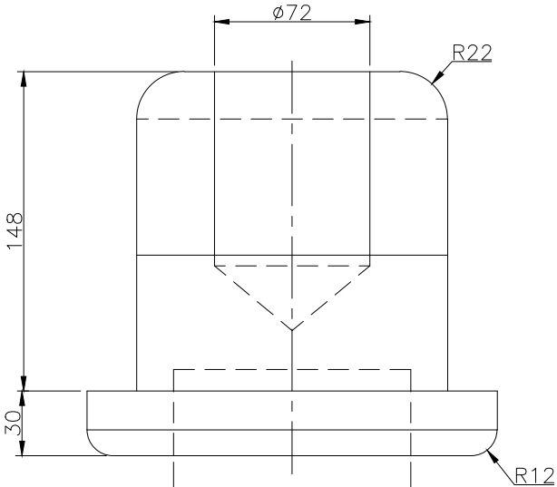
FRONT SCALE 1/3
