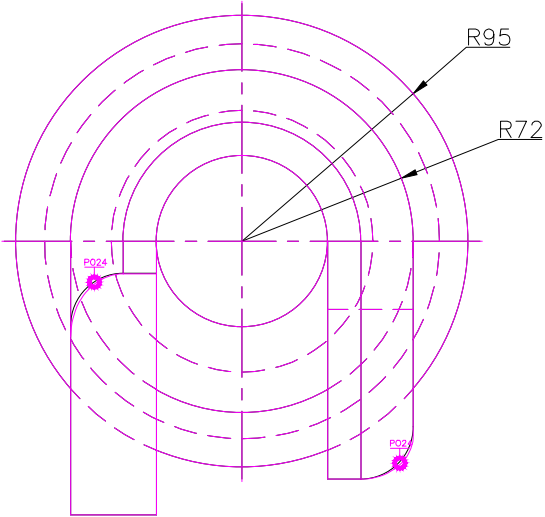
TOP SCALE 1/3
