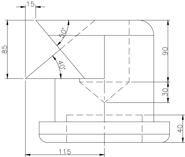
RIGHT SCALE 1/3
