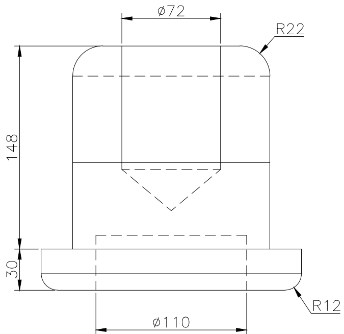
FRONT SCALE 1/3
