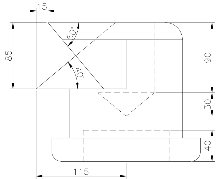
RIGHT SCALE 1/3
