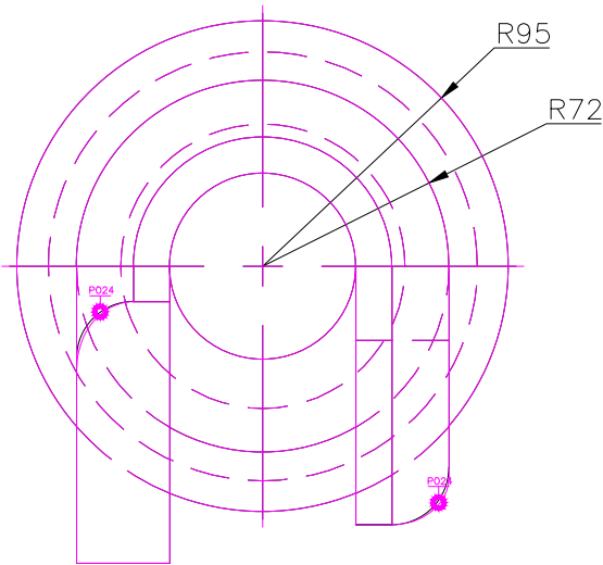
TOP SCALE 1/3
