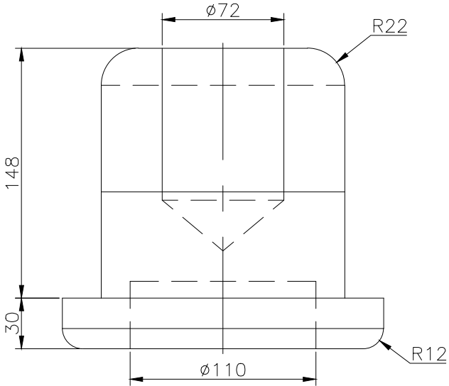
FRONT SCALE 1/3
