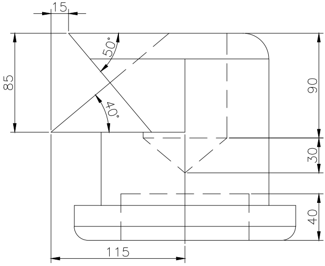
RIGHT SCALE 1/3
