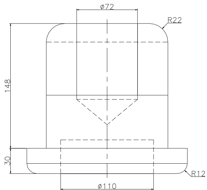
FRONT SCALE 1/3
