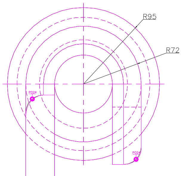
TOP SCALE 1/3
