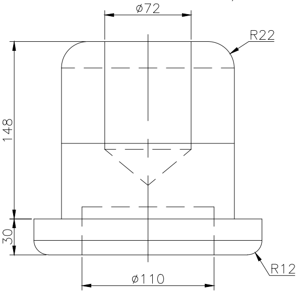
FRONT SCALE 1/3
