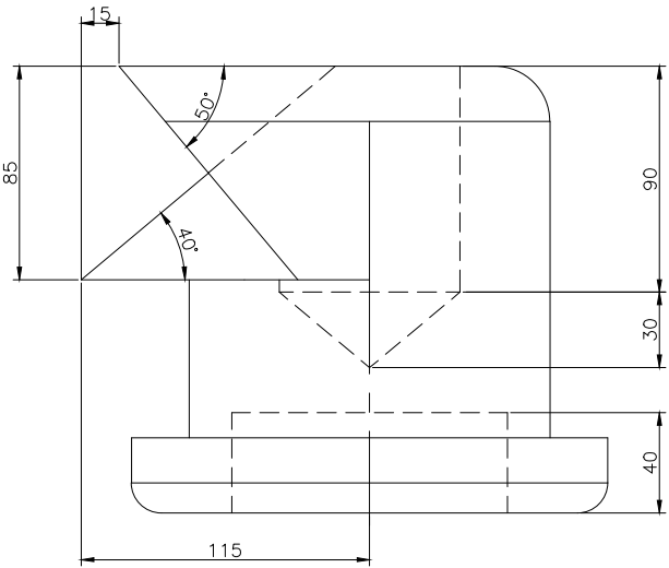
⊕ RIGHT SCALE 1/3
