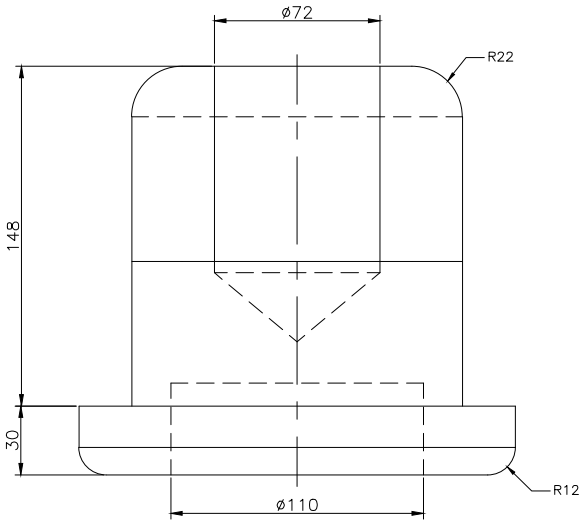
⊕ FRONT SCALE 1/3
