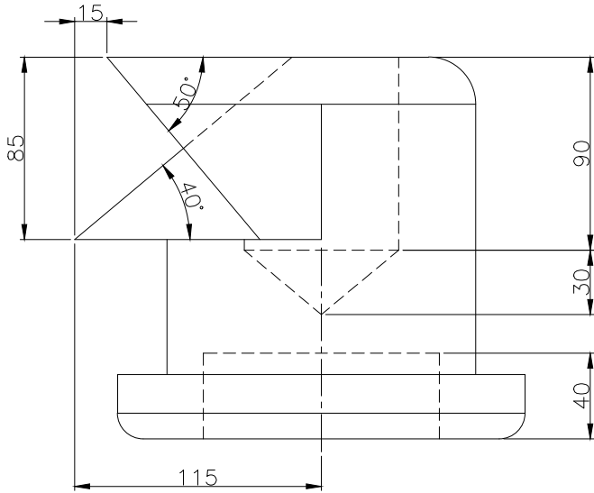
RIGHT SCALE 1/3
