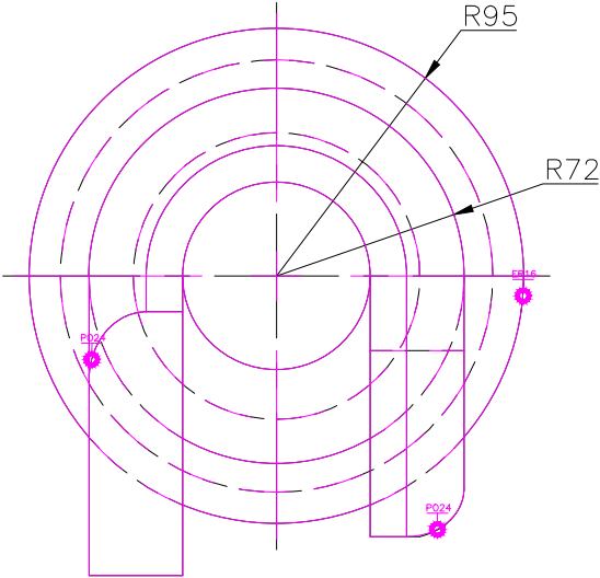
TOP SCALE 1/3
