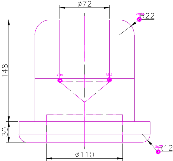
FRONT SCALE 1/3
