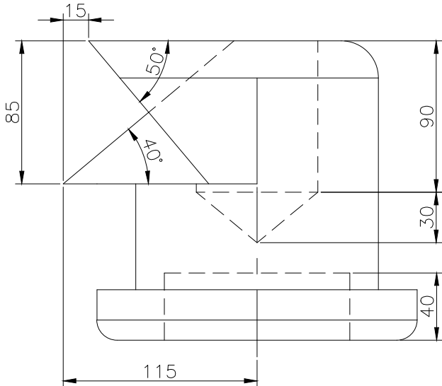
RIGHT SCALE 1/3
