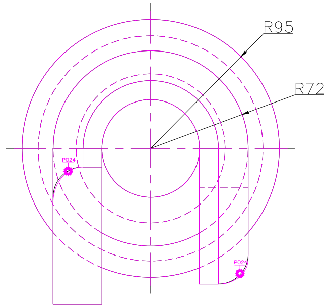
TOP SCALE 1/3
