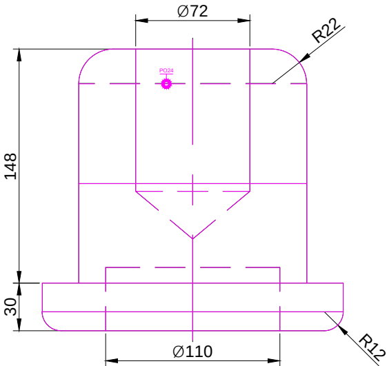
FRONT SCALE 1/3
