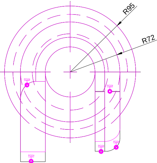
TOP SCALE 1/3
