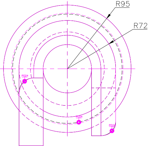
TOP SCALE 1/3
