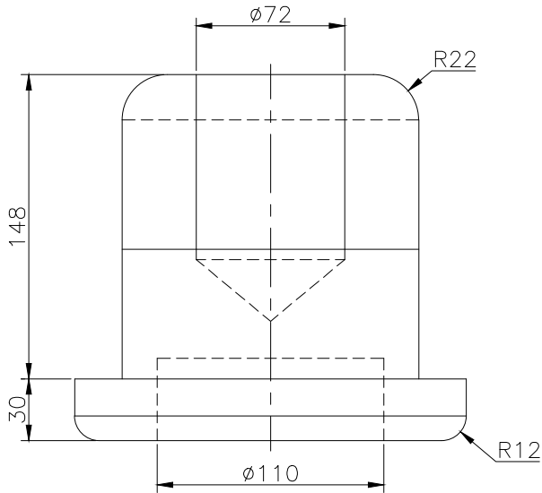
FRONT SCALE 1/3
