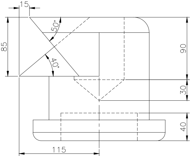
RIGHT SCALE 1/3
