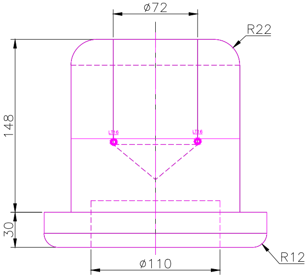
FRONT SCALE 1/3
