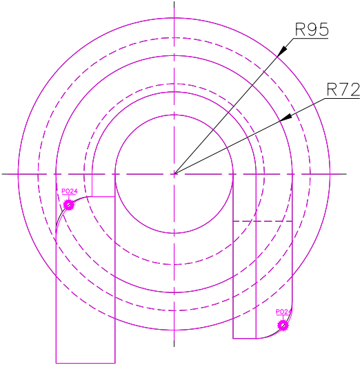
TOP SCALE 1/3
