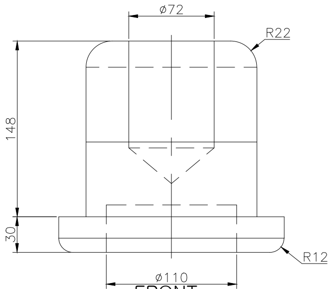
FRONT SCALE 1/3
