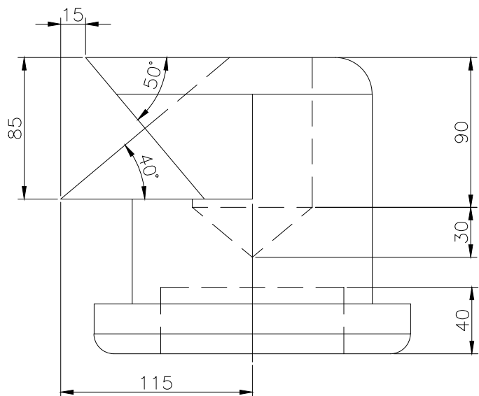
RIGHT SCALE 1/3
