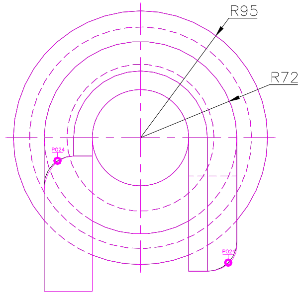
TOP SCALE 1/3
