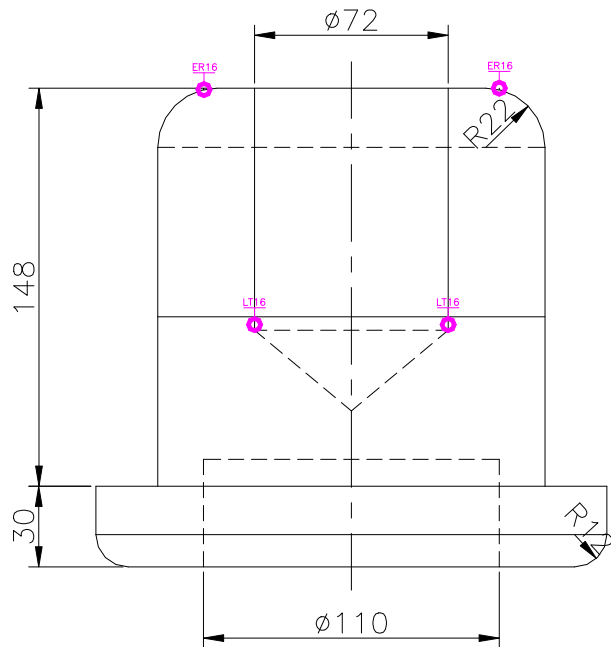
FRONT SCALE 1/3
