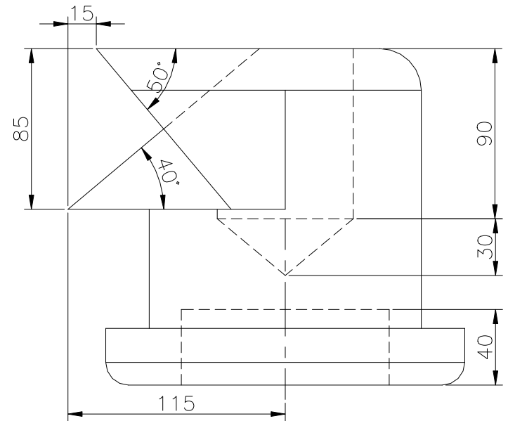
RIGHT SCALE 1/3
