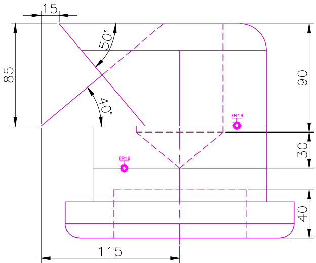
RIGHT SCALE 1/3
