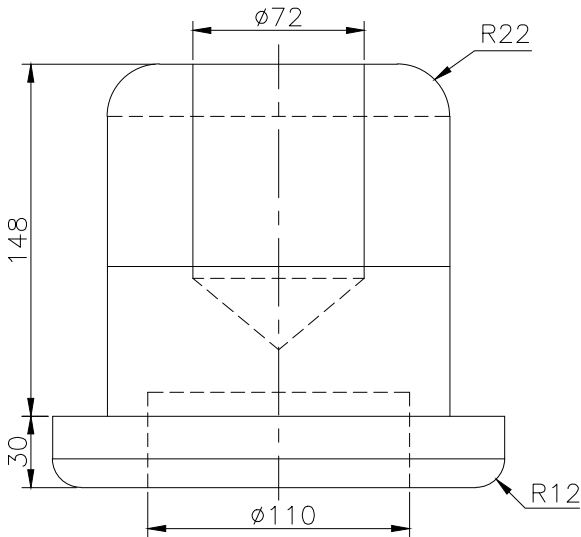
FRONT SCALE 1/3
