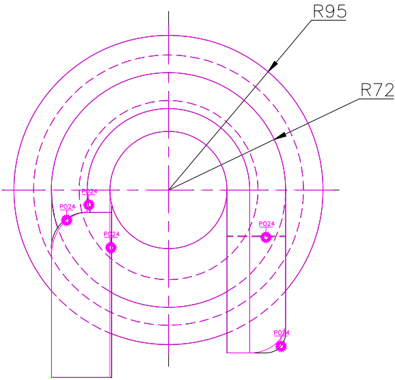
TOP SCALE 1/3
