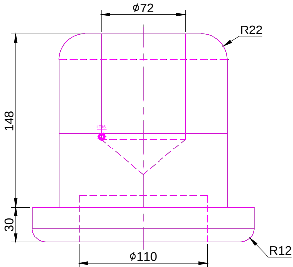
FRONT SCALE 1/3
