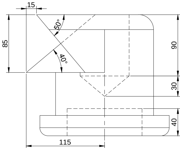
RIGHT SCALE 1/3
