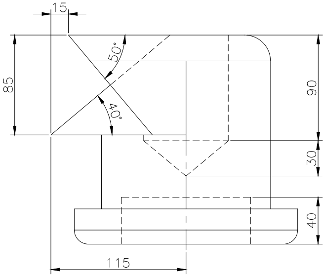
RIGHT SCALE 1/3
