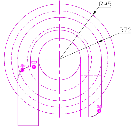
TOP SCALE 1/3
