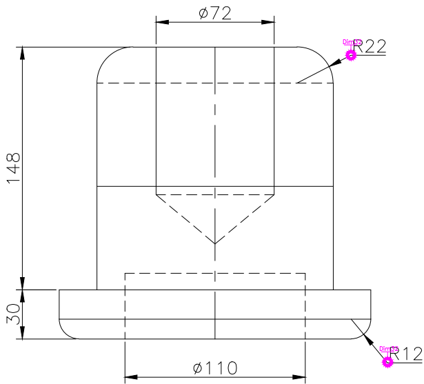
FRONT SCALE 1/3
