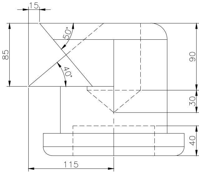
RIGHT SCALE 1/3
