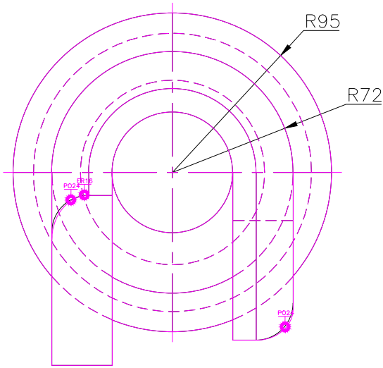
TOP SCALE 1/3
