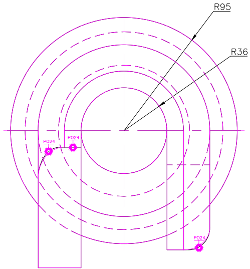
TOP SCALE 1/3
