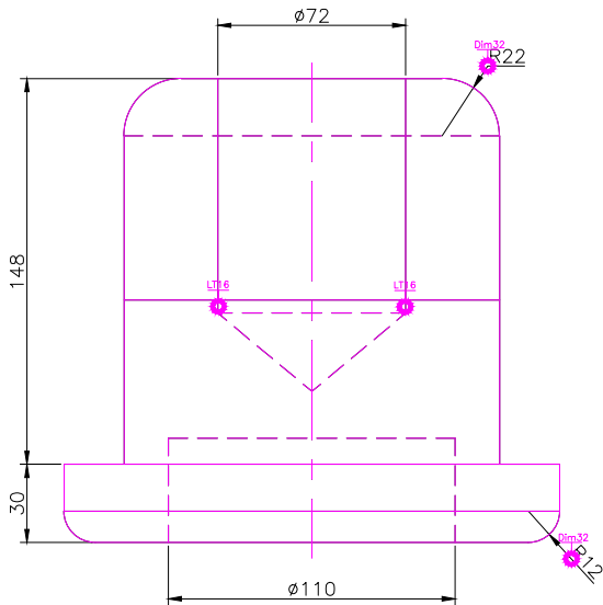
FRONT SCALE 1/3
