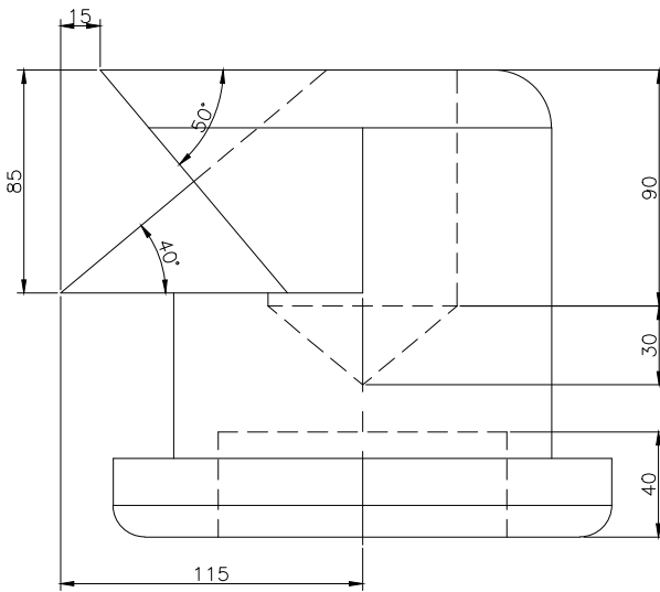
RIGHT SCALE 1/3
